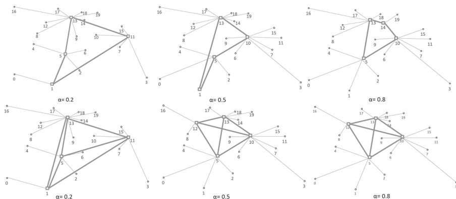
Fig. 1 Optimal networks for CHLP and p HMP with p = 4 and different discount factors
