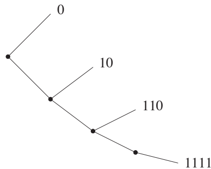
Fig. 4.1. The code tree for the code \mathcal{C}' .
