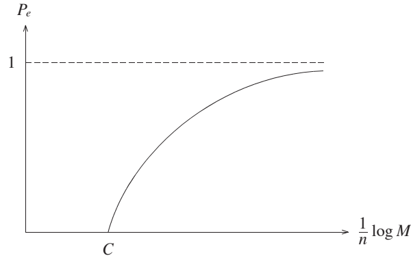
Fig. 7.11. An asymptotic upper bound on P_e .
