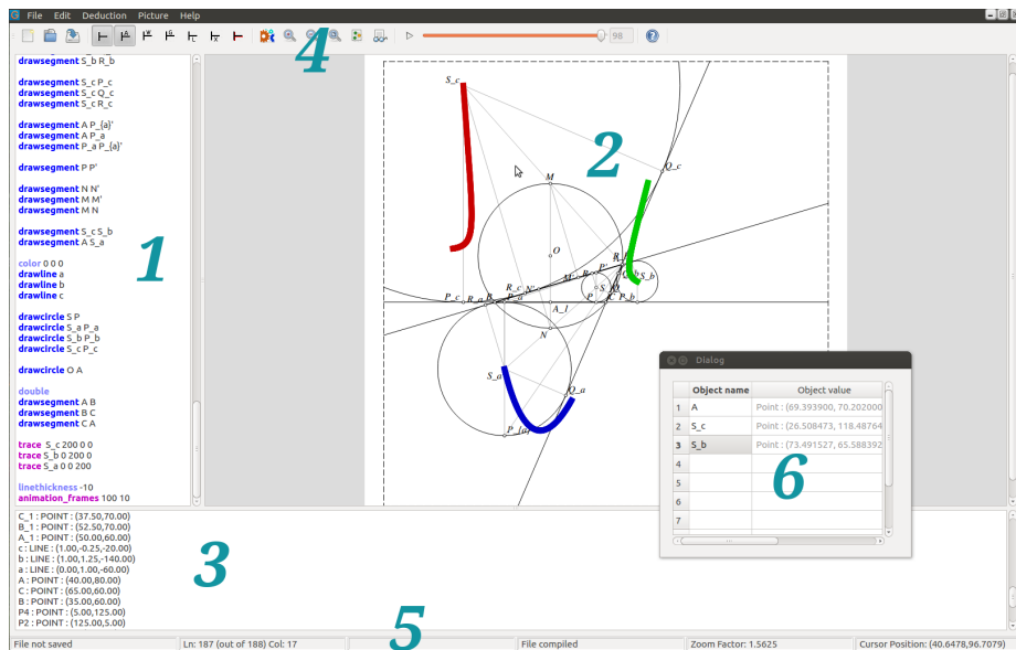
Figure 4.1: Screenshot of gcl-gui
